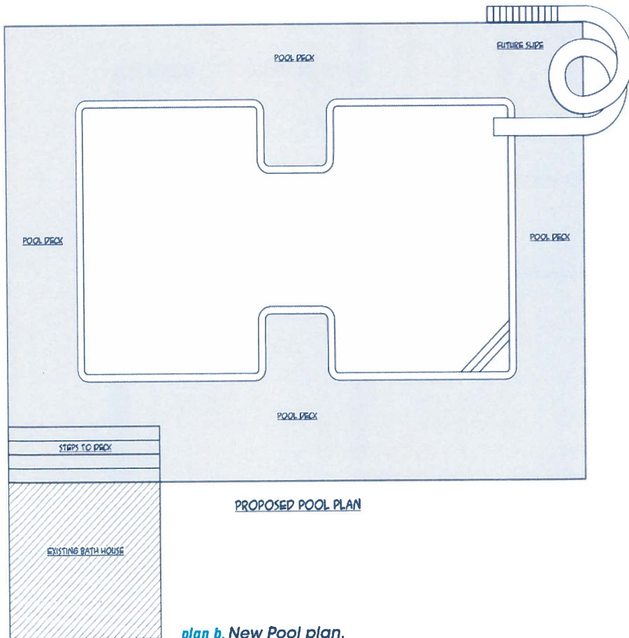
plan b. New Pool plan.
